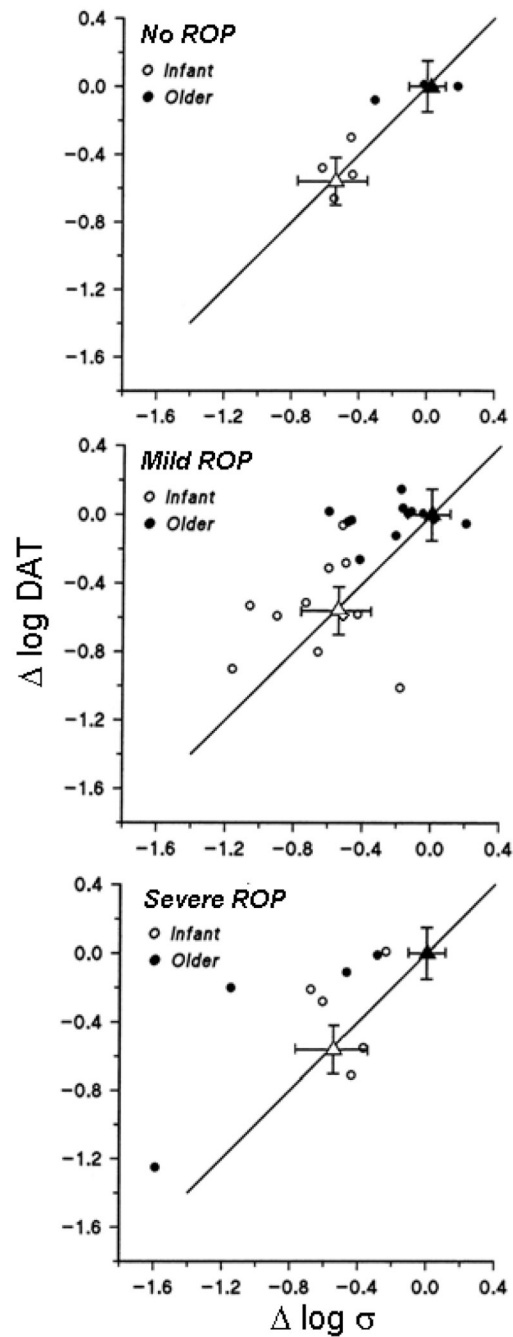
Fig. 4. Deficit in dark adapted peripheral threshold ( \Delta \log \text{DAT} ) plotted as a function of deficit in post-receptor sensitivity ( \Delta \log \sigma ) in preterm subjects with a history of no ROP ( top ), mild ROP ( middle ), and severe ROP ( bottom ). The circles represent data from individual preterm subjects ( open circles – infants; filled circles – older subjects). The triangles indicate the mean ( \pm SEM) for term born 10-week old infants ( open ) and adults ( filled ). The mean normal adult value is at coordinates (0,0). The solid line has a slope of 1.
