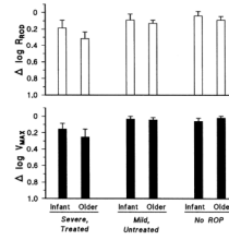
Fig. 3. Mean (SEM) saturated amplitude expressed as the log of the difference from normal for age ( \Delta \log normal). Upper panel: Rod photoreceptor saturated amplitude, R_{ROD} . Lower panel: Post-receptor saturated amplitude, V_{MAX} . The deficit in both amplitude parameters was greatest in severe ROP.
